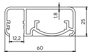
3626 0.978 kg/m
