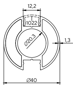
2879 0.755 kg/m
